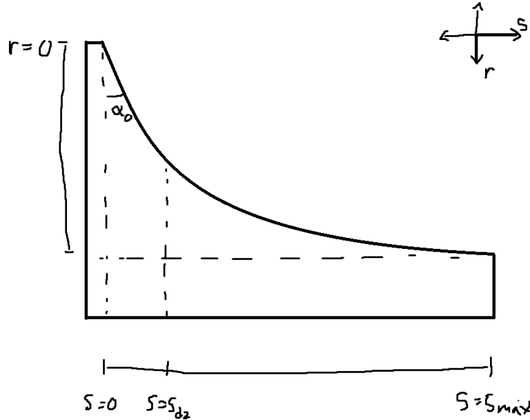
Figure 15: Primary ramp geometry. The flyweight radius is parameterized by r_f(s) , where s is axial travel. The local ramp angle is defined by \tan \alpha_p(s) = dr_f/ds , so steeper profiles (larger dr_f/ds ) redirect a larger fraction of radial force into axial closing force.
