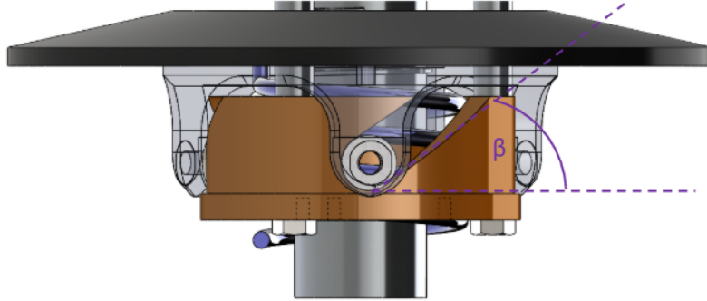
Figure 20: Secondary helix geometry. Tangential force generated by shaft torque is redirected into axial force. The projection introduces a factor 1/\tan \alpha_s , which equals r_h d\theta_s/ds by definition of the helix mapping. TODO: Add a point with forces (FBD)
