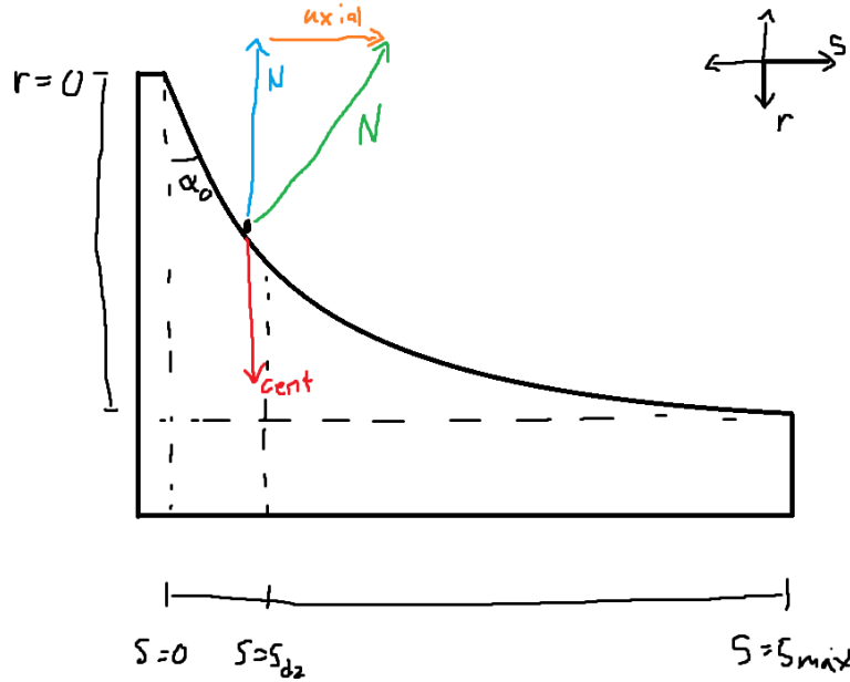
Figure 18: Primary ramp geometry. Radial centrifugal force is redirected into axial force through the ramp. The projection introduces a factor of \tan \alpha_p , which equals dr_f/ds by definition of the ramp slope.
